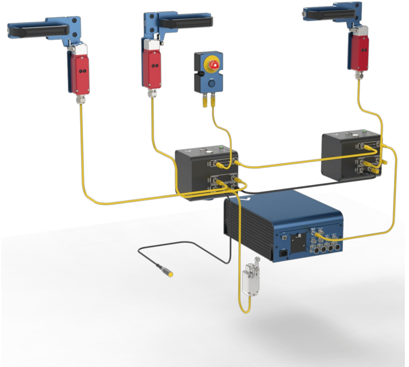
Figure 5: Daisy-chaining Access Request Modules
