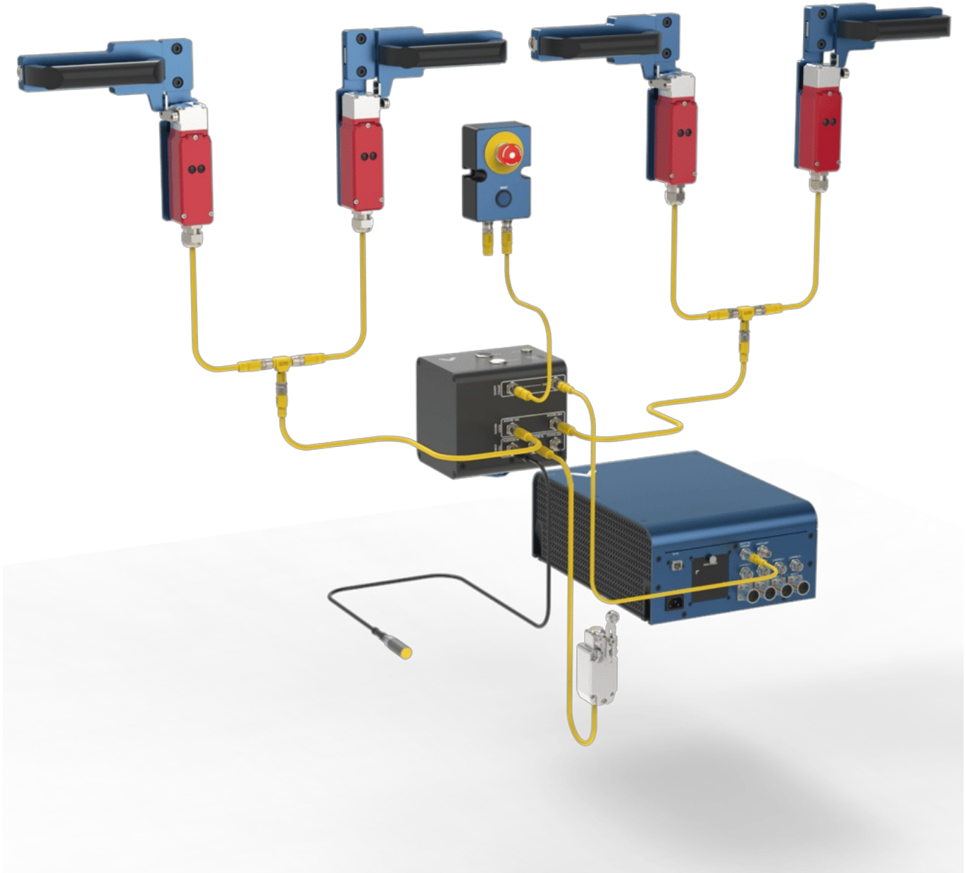
Figure 4: Access Request Module with 4 guardlocks
