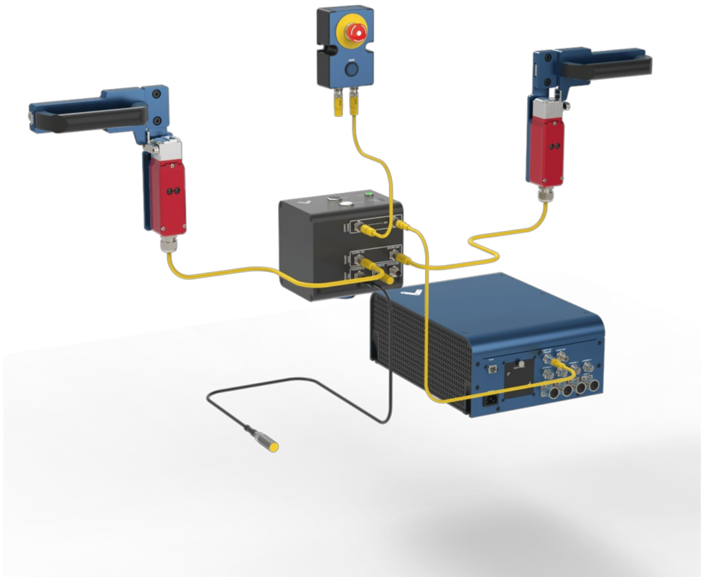
Figure 7: Access Request Module with 2 guardlocks
