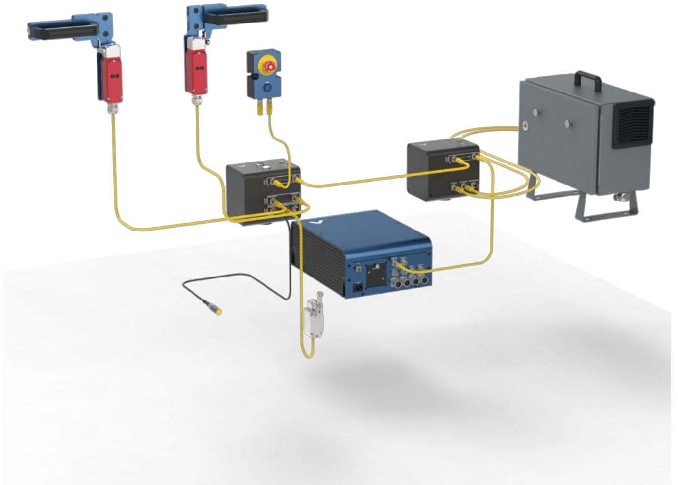
Figure 6: Access Request Module with Robot Safety Module
