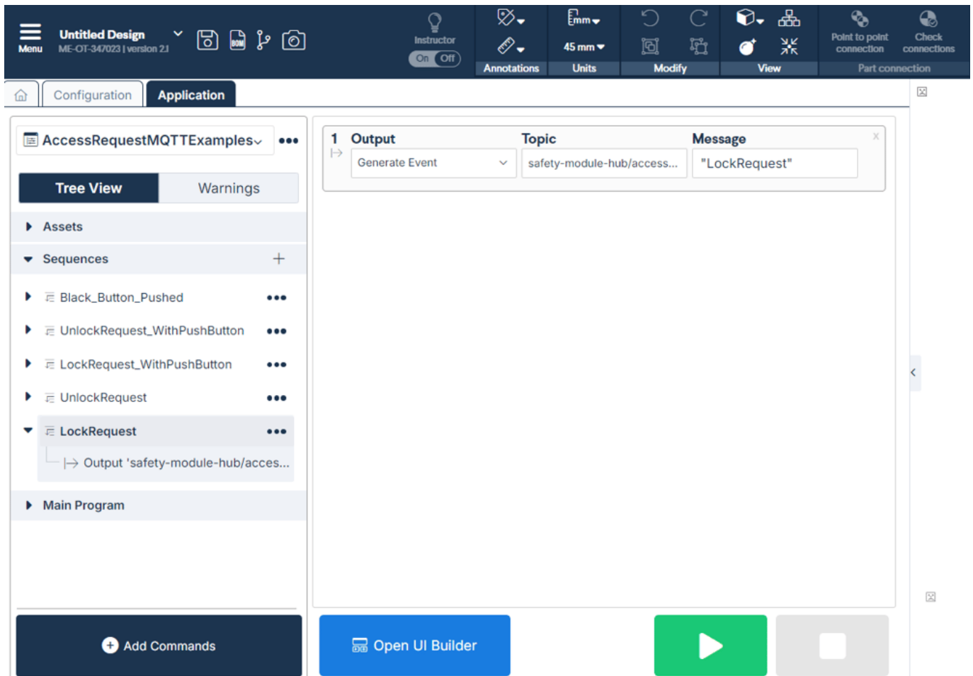
Figure 9: MachineLogic example to handle a lock request from the Access Request Module
