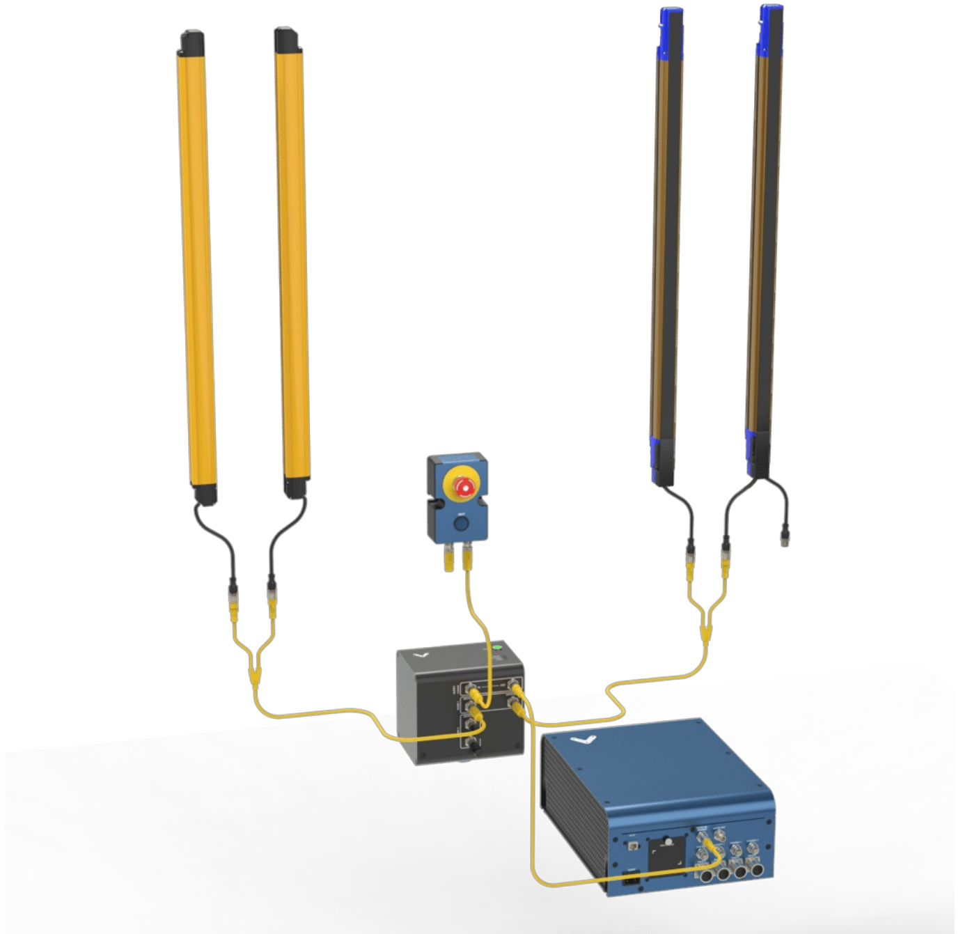
Figure 5: Mode Switching Safety Module wiring diagram for Keyence & Datalogic Light Curtains
